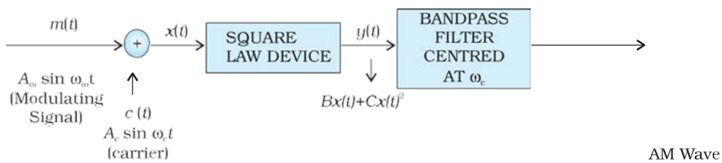
FIGURE 15.10 Block diagram of a simple modulator for obtaining an AM signal.
